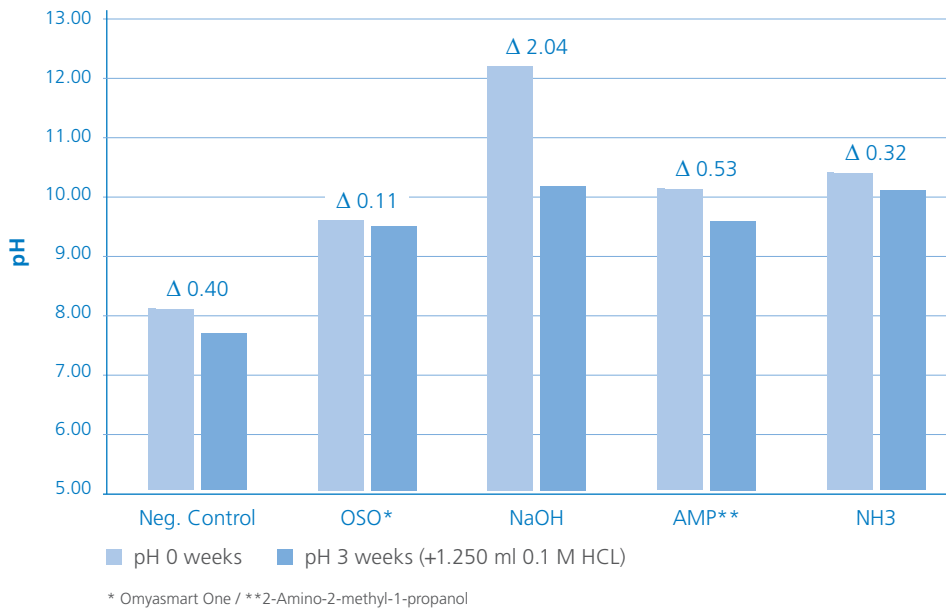
Figure 1: PH stability of Omyasmart One compared to other neutralizing agents in an Omycarb paint dispersion. Due to its special properties, Omyasmart One establishes high salt and keeps the optimal high PH stable for the long shelf life of the paints and coatings. Compared to conventional neutralizing agents, Omyasmart One has the best buffering effect.
