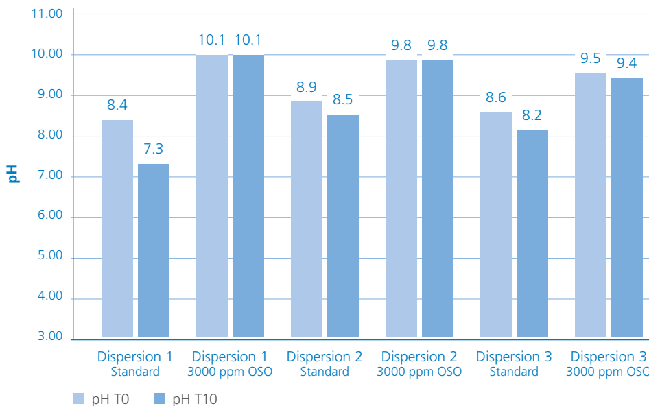
Figure 2: This picture shows the pH stability of Omyasmart One in different paint dispersions in contrast to the standard (without OSO) over 10 weeks. Paint Formulations with Omyasmart One show a high pH-stability. Independent of the paint dispersion, the paints comprising Omyasmart One show more stability in comparison to paint dispersions containing other neutralizing agents.
