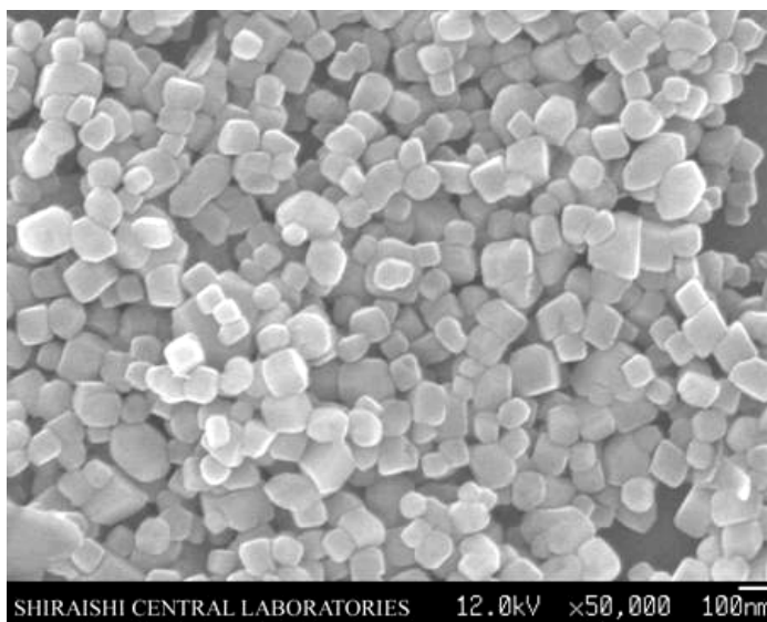
SEM Image × 50,000
